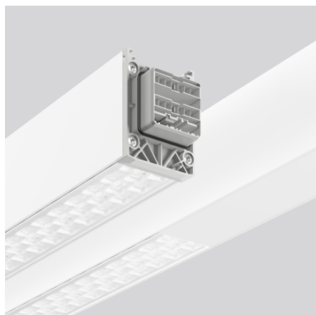
Lichtband 4051859610755 L 2291, B 58, H 76
