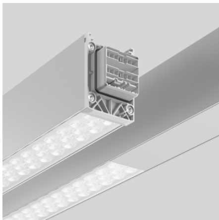
Lichtband 4051859569510 L 4547, B 58, H 76
